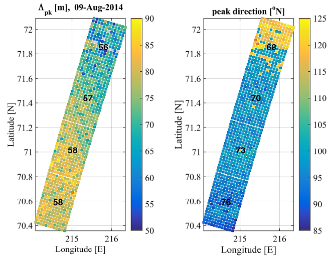
Fig. 2. Spatial heterogeneity of dominant wave length \lambda_{pk} (left) and dominant wave direction (right). Colour fields show results retrieved from TerraSAR-X Stripmap images, black numbers give Wavewatch III model results.
