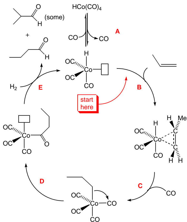
Heck-Breslow mechanism for cobalt-catalysed hydroformylation .
