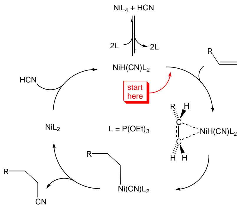
Mechanism for nickel-catalysed hydrocyanation .
