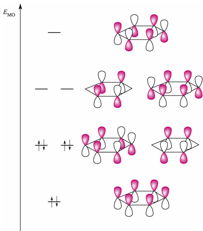
The \pi -molecular orbitals of \text{C}_6\text{H}_6 .
