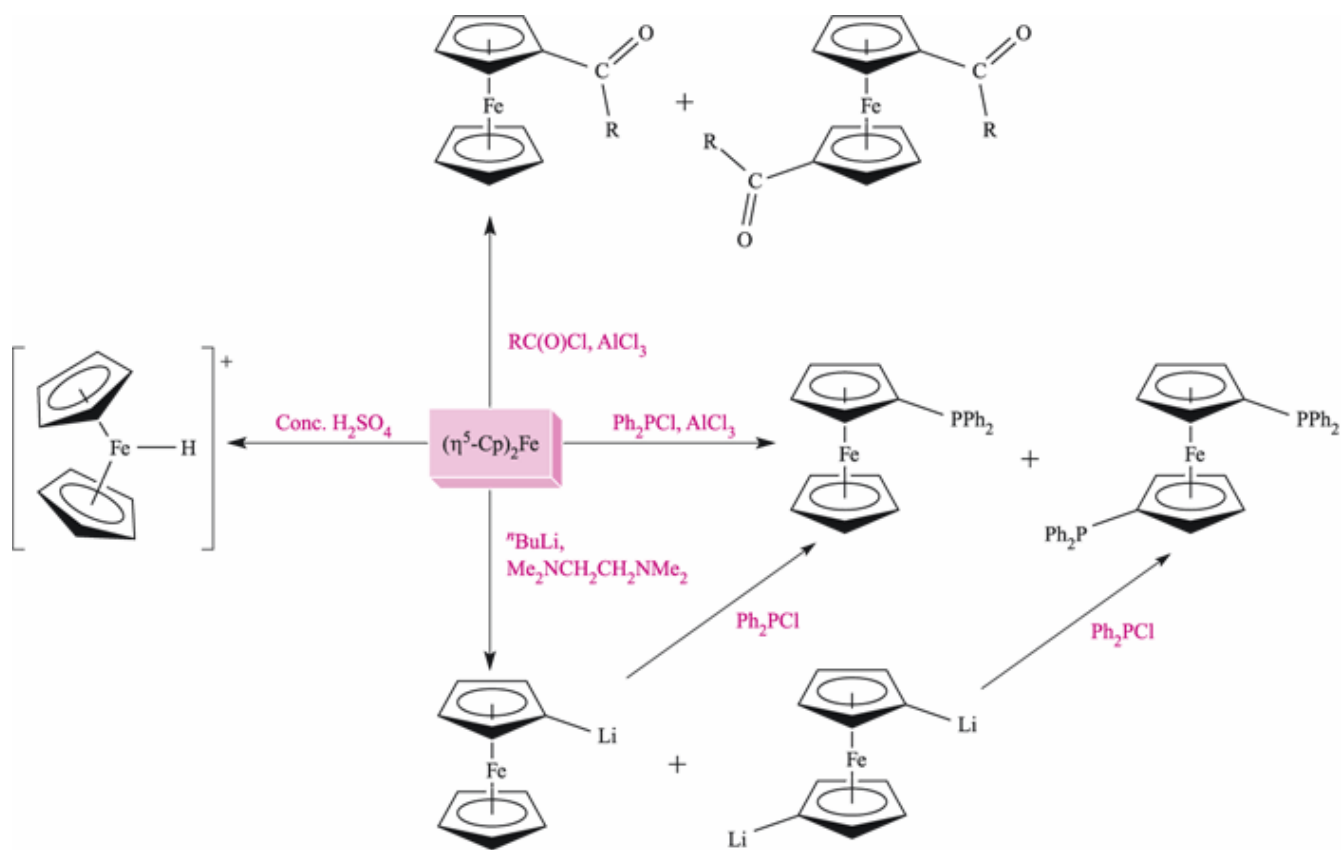
Selected reactions of ferrocene, (\eta^5\text{-C}_5\text{H}_5)_2\text{Fe} .
