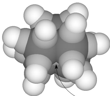
\text{Fe}_5\text{C}(\text{CO})_{15} space-filling
