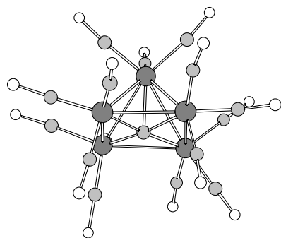
\text{Fe}_5\text{C}(\text{CO})_{15} ball-and-stick
