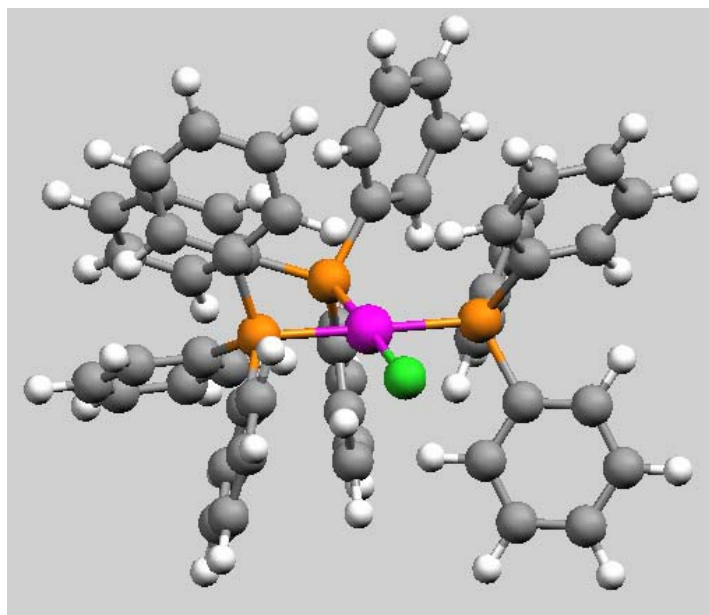
Figure 9.2 Wilkinson's catalyst, \text{RhCl}(\text{PPh}_3)_3 .
