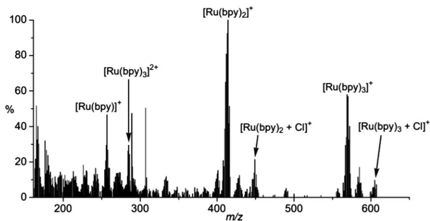
FIGURE 7 LSIMS spectrum of [Ru(\text{bipyridine})_3]Cl_2 in a 3-nitrobenzyl alcohol matrix. Adopted with permission from Gross and Caprioli 20
