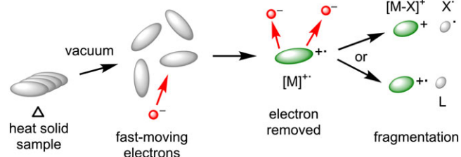
FIGURE 1 Cartoon showing the EI process. The neutral sample is heated under vacuum, driven into the gas phase, and ionized with electrons accelerated to 70 eV. The electrons ionize and fragment the target molecule
