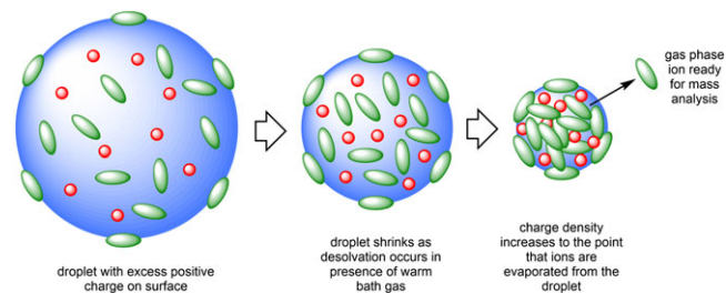
FIGURE 10 Cartoon showing the ESI process. Solution-phase ions are passed through a charged capillary, and the solution separates into tiny droplets from which the solvent is evaporated. The excess charges arrange themselves on the surface, and as the charge density increases, ions are evaporated into the gas phase
