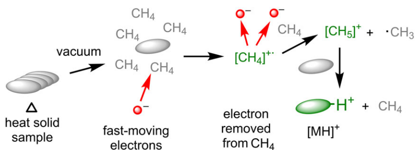
FIGURE 3 Cartoon showing the CI process. The neutral sample is heated under vacuum, driven into the gas phase in the presence of a reagent gas (typically methane) and the reagent gas is ionized with electrons accelerated to 70 eV. The resulting [CH_4]^+ ions react with CH_4 to make \cdot CH_3 radicals and [CH_5]^+ , and the latter protonates gas phase sample molecules to make [MH]^+ ions
