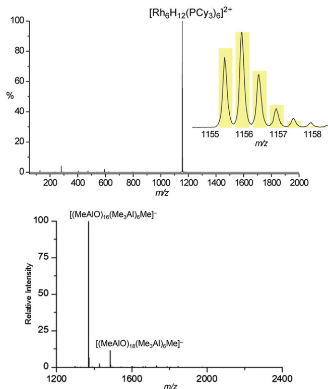
FIGURE 11 ESI mass spectra of a dicationic rhodium cluster compound (top, with isotope pattern inset) and of an anionic methylalumoxane oligomer (bottom). Note the lack of fragmentation which is characteristic of ESI, and in the dicationic example, preservation of the original charge state, evident from the peaks in the isotope pattern being m/z 0.5 apart. Spectra reproduced with permission from Brayshaw et al and Zijlstra et al 34,35
