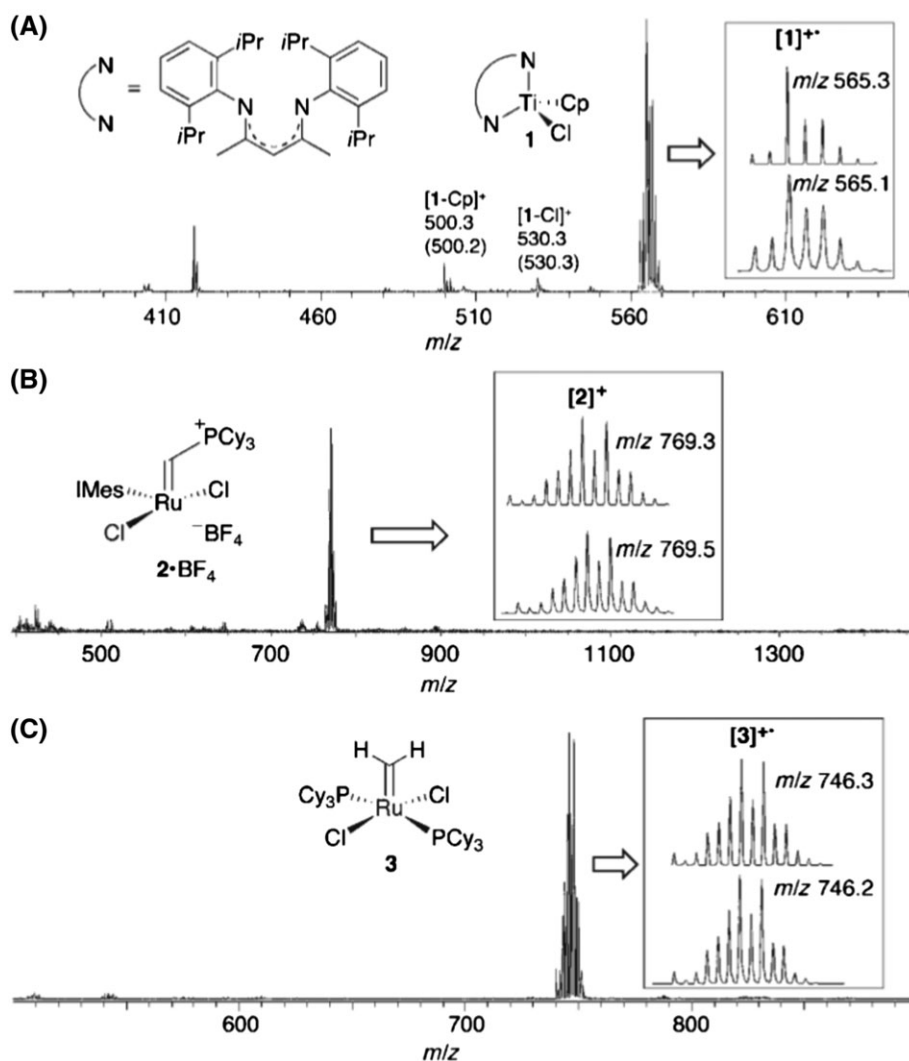
FIGURE 9 MALDI mass spectra of isolated complexes. A, An oxophilic Ti^{III} complex (pyrene matrix); B, the Piers metathesis catalyst (pyrene matrix); C, a first-generation Grubbs catalyst (anthracene matrix). Labels give found (calculated) m/z values. Insets show isotope patterns for the molecular ions (top: simulated, bottom: observed). Cp = C_5H_5 , IMes = N,N' -bis (mesityl)imidazol-2-ylidene, Cy = cyclohexyl. Spectra reproduced with permission from Eelman et al 23
