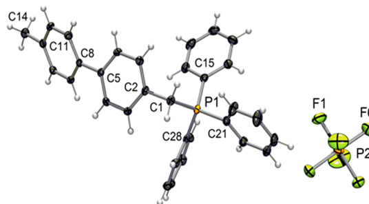
Figure 1. X-ray crystal structure of [4,4'-MeC_6H_4C_6H_4CH_2PPh_3]-[PF_6] . The new C–C bond is between C5 and C8. The angle between the benzyl and tolyl rings is 26.76(8)^\circ , and the bond angles and lengths were similarly ordinary.
