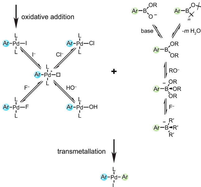
Scheme 3. Proposed Set of Equilibria Resulting from the Various Palladium and Boron-Containing Species Considered Herein a
