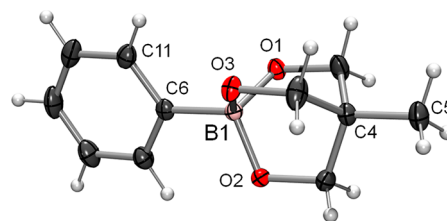
Figure 8. X-ray crystal structure of [NEt 4 ][PhB(O 3 C 5 H 9 )]. The tetraethylammonium cation and solvent of crystallization have been excluded for clarity. The compound was characterized crystallographically as the dihydrate, but all samples used in the MS studies were dried until no water was observable in the 1 H NMR spectrum (see Supporting Information). Key bond lengths and angles: B1–C6 1.6142(16) Å; B1–O average 1.494 Å; C6–B1–O average 110.5°; B1–O–C average 111.2°.
