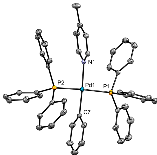
Figure 14. X-ray crystal structure of [(Ph 3 P) 2 Pd(Ph)(C 6 H 7 N)] + [OTf] - . The triflate anion, solvent of crystallization (CH 2 Cl 2 ), and hydrogens have been excluded for clarity. Key bond lengths and angles: Pd1–C7 2.0196(19) Å, Pd1–N1 2.1244(16) Å, C7–Pd1–N1 176.46(7)°, N1–Pd1–P2 89.85(4)°, N1–Pd1–P1 92.81(4)°, C7–Pd1P2 86.77(6)°, C7–Pd1–P1 90.45(6)°.
