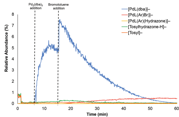
Fig. 5 PSI-ESI-MS monitoring of the oxidative addition of bromotoluene to Pd(sSPhos)(dba).
