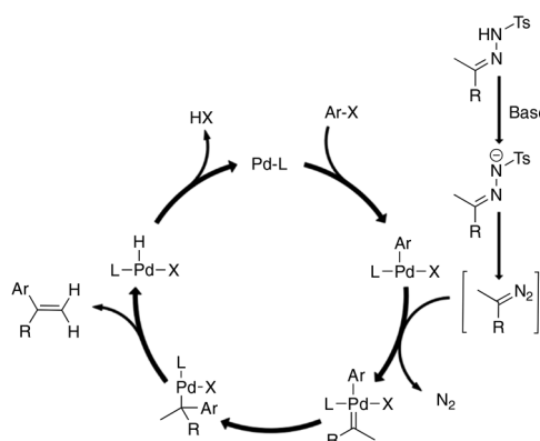
Fig. 1 Proposed catalytic cycle of the reaction between N -tosylhydrazones and aryl halides. 19
