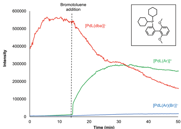
Fig. 6 Negative ion mode monitoring of [\text{Pd}(\text{sSPhos})(\text{dba})]^- and [\text{Pd}(\text{sSPhos})(\text{Ar})(\text{Br})]^- overlaid with positive ion mode monitoring of [\text{Pd}(\text{SPhos})(\text{Ar})]^+ . Inset: Structure of SPhos ligand.
