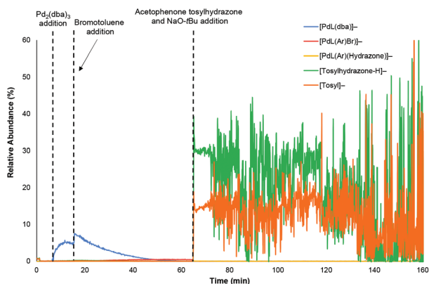
Fig. 7 Complete PSI-ESI-MS monitoring trace of the Pd-catalyzed reaction between acetophenone tosylhydrazone and bromotoluene.
