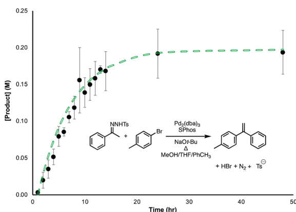
Fig. 2 1 H-NMR reaction monitoring using final reaction conditions based on screen (inset) over 48 hours, error bars indicate triplicate experiments. Dashed green line represents first order fit. Conditions: 1% [Pd], 2% SPhos, 0.003 mol acetophenone tosylhydrazone, 0.003 mol bromotoluene, 0.0067 mol NaOt-Bu, 70 °C.
