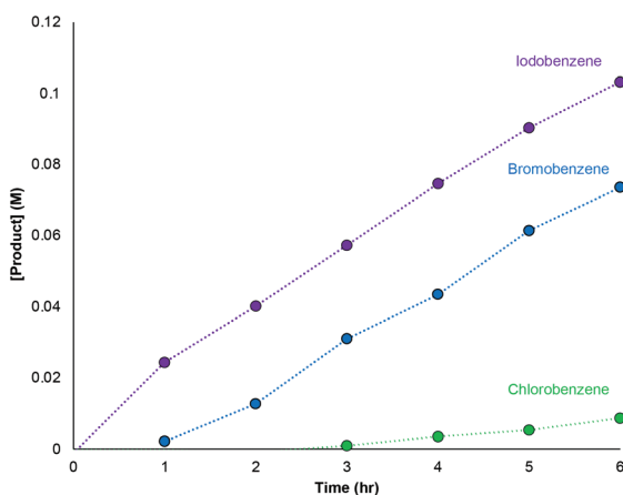
Fig. 4 Effect of aryl halide on the initial rate of product formation. Conditions: 1% [Pd], 2% SPhos, 0.003 mol acetophenone tosylhydrazone, 0.003 mol ArX, 0.0067 mol NaOt-Bu, 70 °C.
