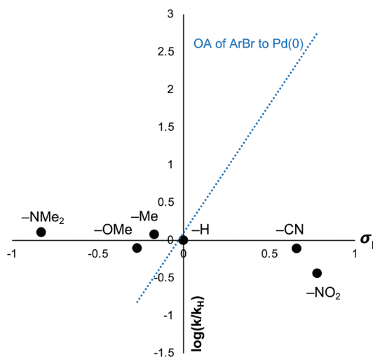
Fig. 3 Hammett plot of \log(k/k_H) vs. Hammett parameter ( \sigma_p ) 38 for para -substituted aryl bromides as labelled. k represents the initial reaction rate of each substituent, and k_H represents the initial reaction rate of the H-substituted substrate. The trendline represents the oxidative addition of para -substituted aryl bromides to Pd(0) as reported by Lu et al. 39
