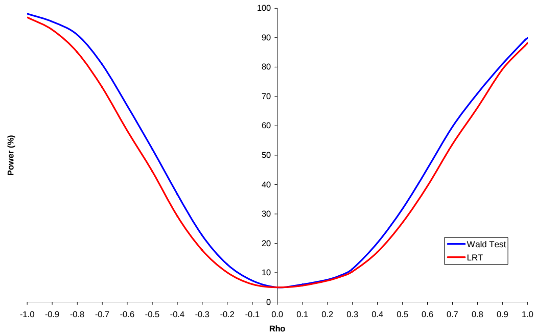
Power Curves for Wald Test & LRT H0: Serial Independence vs H1: AR(1) (Tests have been "size-adjusted" to 5%)
