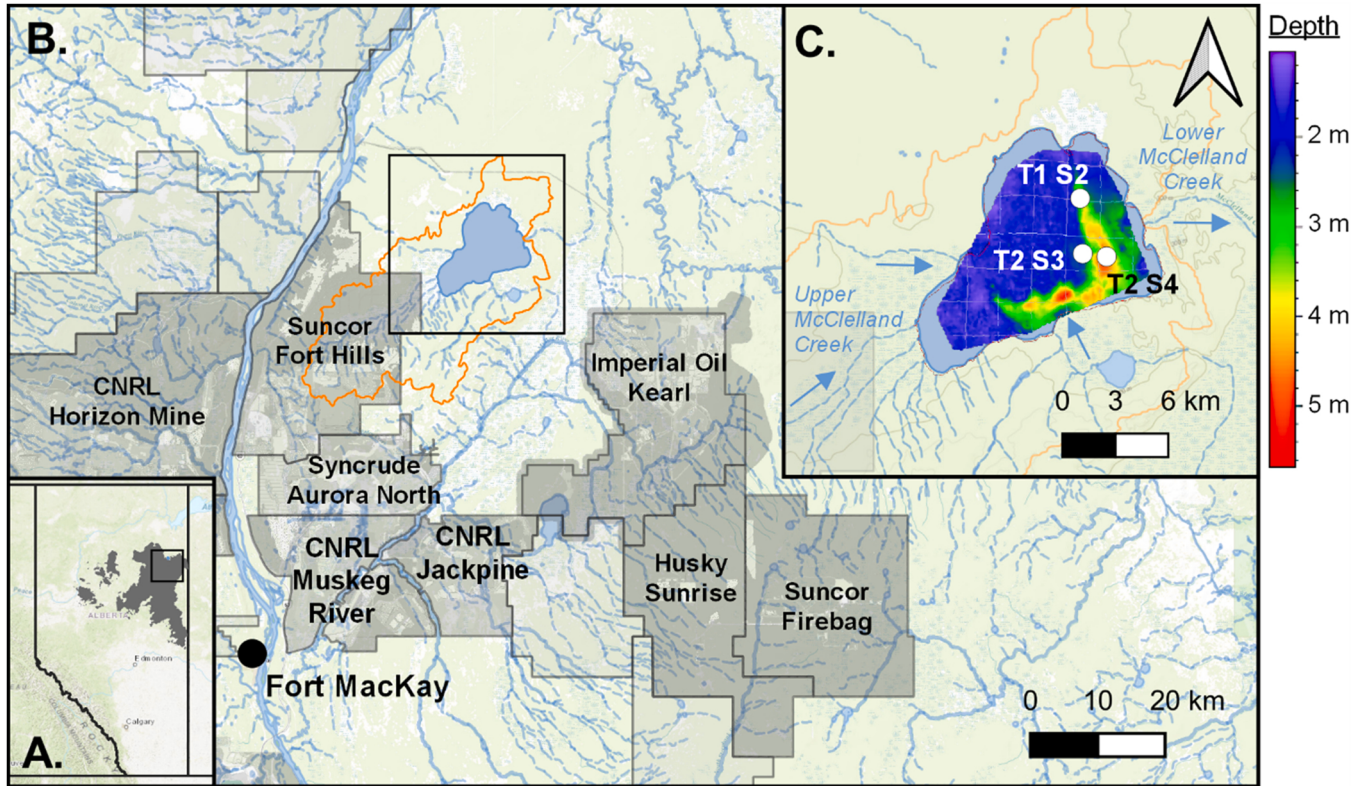
Fig. 1. (A) Location of McClelland Lake within the oil sands deposits (dark grey) of northern Alberta; (B) The McClelland Lake watershed (orange outline), with local active oil sands projects (medium grey fill) and inactive/prospective projects (light grey outline) indicated; and (C) McClelland Lake, including lake depth (colour gradient), inflows to the west and south, and the outflow to the east (blue lines). Locations of the three sediment coring sites reported in this paper are indicated with white circles. (For interpretation of the references to colour in this figure legend, the reader is referred to the web version of this article.)
