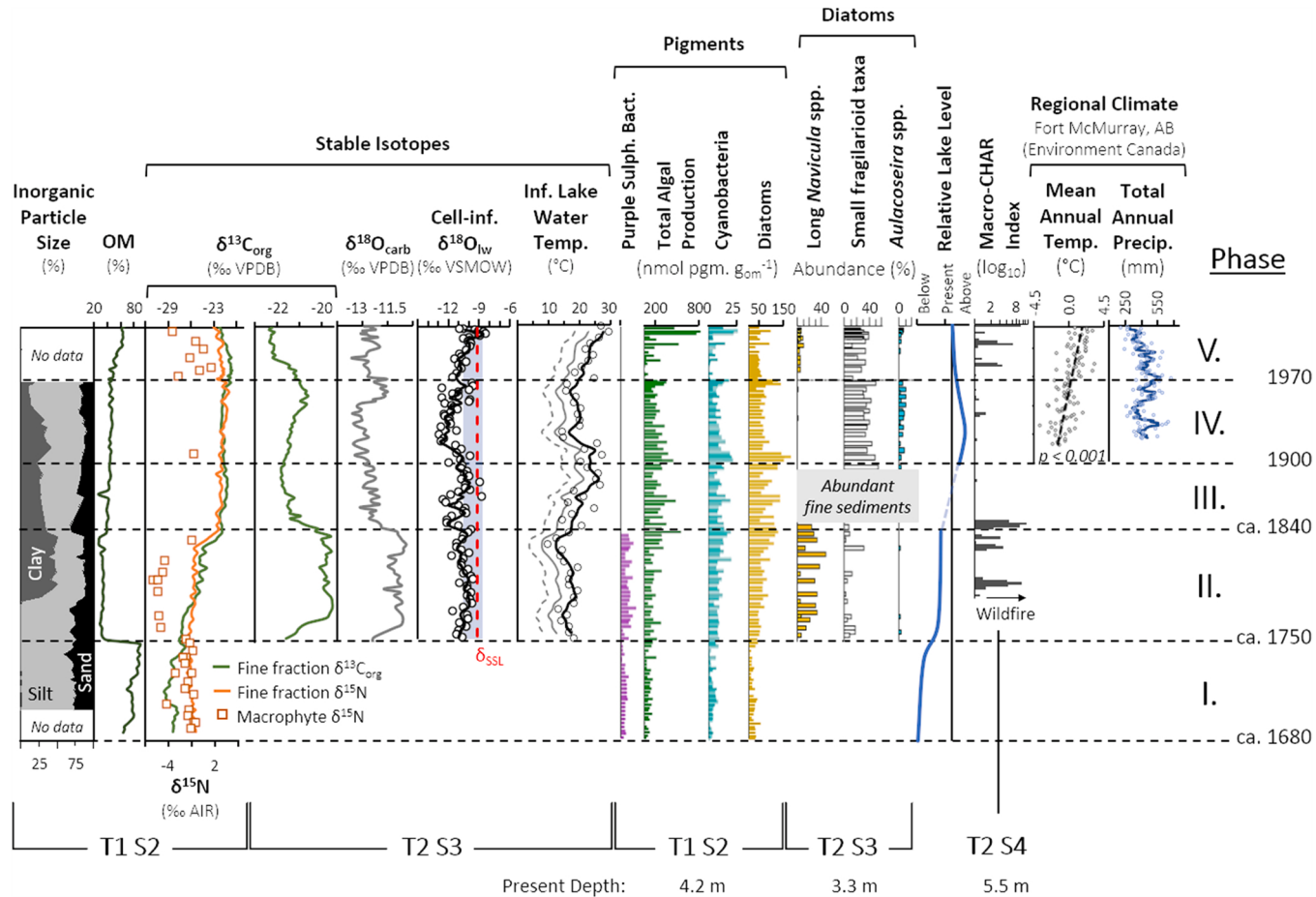
Fig. 3. Summary of the paleolimnological reconstruction at McClelland Lake, AB, highlighting stratigraphic profiles of key variables measured in indicated sediment cores as well as external climatic data (Environment Canada, Fort McMurray, AB, stations 3062693, 3062695, 3062696). Nitrogen isotope ratios ( \delta^{15}\text{N} ) are presented for the sediment fine fraction ( < 250 \mu\text{m} ; orange solid line) and coarse macrophyte fragments (orange squares). Organic carbon isotope ratios ( \delta^{13}\text{C}_{\text{org}} ) for the sediment fine fraction organic matter are shown for two cores using green solid lines. Three-point running mean cellulose-inferred \delta^{18}\text{O}_{\text{lw}} is shown using a black solid line while individual values are shown using open circles. Superimposed on this plot is the range of measured lakewater \delta^{18}\text{O} values (vertical grey-blue bar), and the estimated contemporary terminal basin isotopic steady-state value ( \delta_{\text{SSL}} ; vertical red dashed line) from Remmer et al. (2018). Inferred lake-water temperature was calculated under three scenarios: 1) following Leng and Marshall (2004) and the three-point running mean using a black line; 2) under the assumption carbonates precipitated in more isotopically depleted water (grey solid line); and 3) assuming carbonates were affected by kinetic fractionation in more isotopically depleted water (grey dashed line; Rozanski et al., 2010). Relative lake level was semi-quantitatively inferred based on macrophyte remains, diatom community composition, stable isotope ratios, and inorganic particle size distributions. Significant rise of regional mean annual temperature is shown using a black dashed line, with individual data points shown with open circles. Total annual precipitation is shown using open blue circles and the three-point running mean is shown using a blue solid line. The present water depth of each coring site is indicated along the bottom of the figure. Five hydroecological phases were delineated through qualitative inspection of stratigraphic variations and numerical analyses of all measured sedimentary variables separately for all cores used in this study. (For interpretation of the references to colour in this figure legend, the reader is referred to the web version of this article.)
