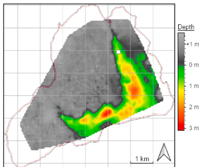
Fig. 4. Bathymetric map of McClelland Lake showing reconstructed low water levels during Phase I (ca. 1695 – 1750), as inferred by macrophyte remains and stable isotope measurements. Sediment core location T1 S2 is indicated using the white circle, on which this paleo-lake level reconstruction is mainly based. Grey areas indicate presently submerged regions of the lake that were likely exposed during this period. White areas within the lake's perimeter indicate regions for which bathymetric data were not available. Graticule is composed of 1 \times 1 km squares.
