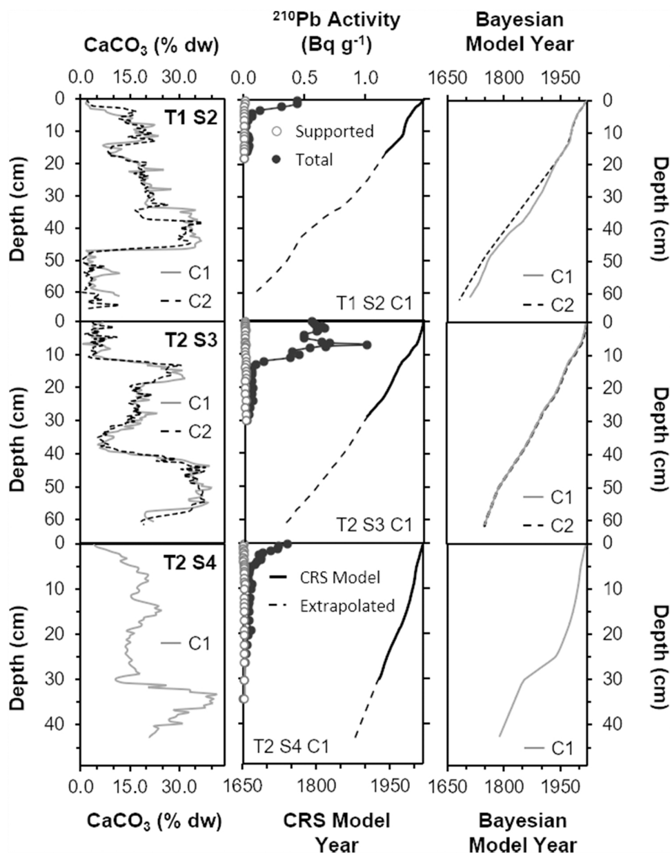
Fig. 2. Wiggle-matched carbonate content (left), total ^{210}\text{Pb} activities (center, dark grey circles) and supported ^{210}\text{Pb} activities (center, open light grey circles), CRS model ages (center, black line) and extrapolated age estimates (center, black dashed line), and Bayesian age-depth models (right) for the three coring sites used in this study.
