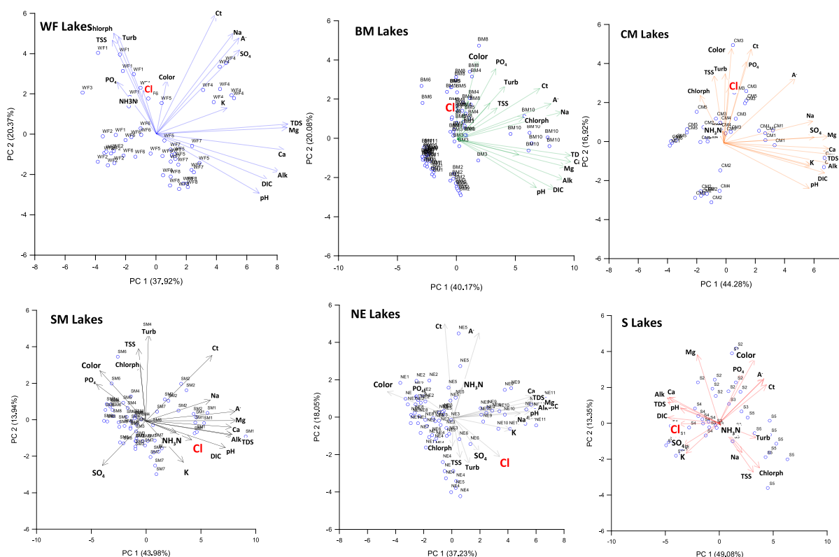
Fig. 5. PCA biplot of RAMP lakes subregions. Each lake number is represented within the symbol. Increments of pH, DIC, alkalinity, base cations (Ca, Mg and K) and TDS are observed along the PC1 in WF, SM, BM, CM and NE. PC2 shows variations of chlorophyll, color, TSS, turbidity \text{PO}_4 and Ct on the same lake subregions. The S lakes in the Canadian Shield show a opposite direction distribution of the variables mentioned before along the PC1 and PC2. To note the variability of the ion chloride assumed to behave conservatively.
