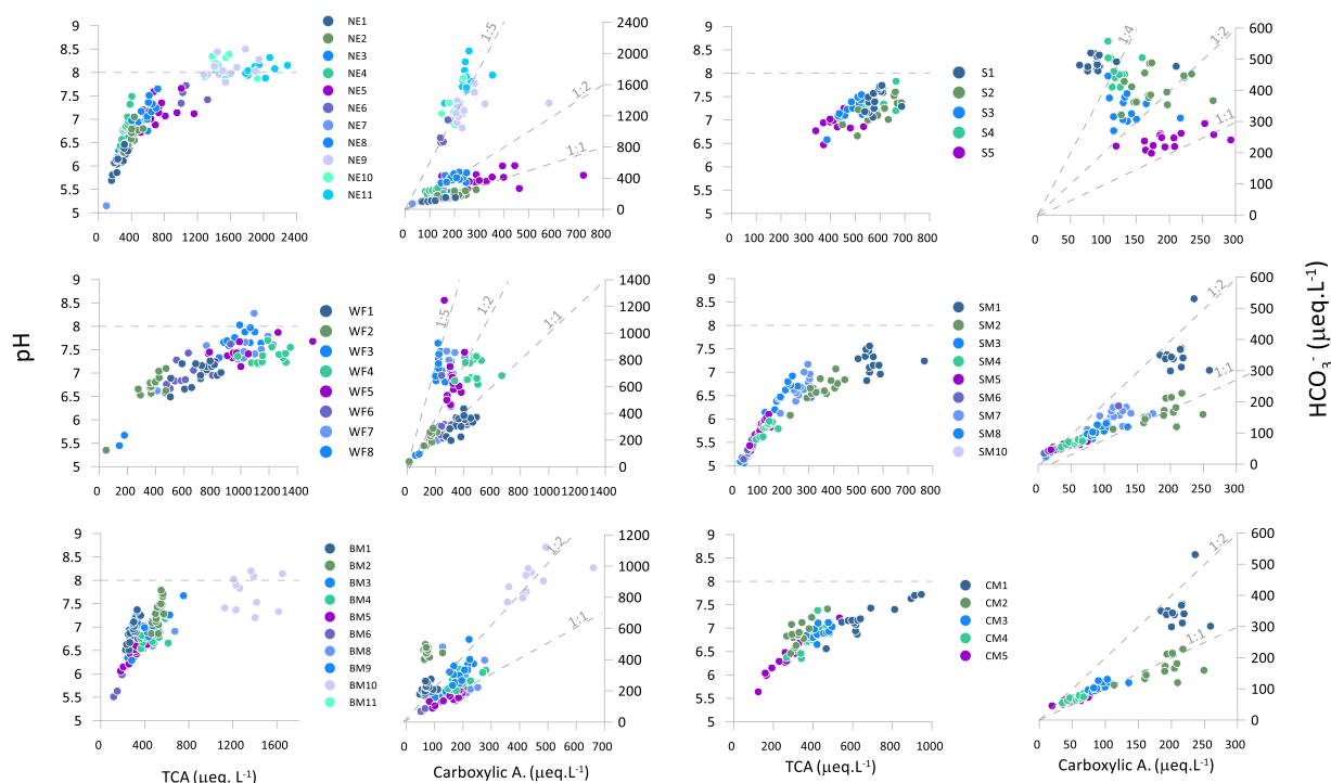
Fig. 7. Relative \text{HCO}_3^- and ionized carboxylic acid ( \text{A}^- ) contribution to the total carbonate alkalinity (TCA) in the RAMP lakes. To note the higher contribution from \text{HCO}_3^- to some lakes in the NE, WF subregions closer to oil sands operations and the lower contribution at the SM and CM lakes further away from the oil sands operations.
