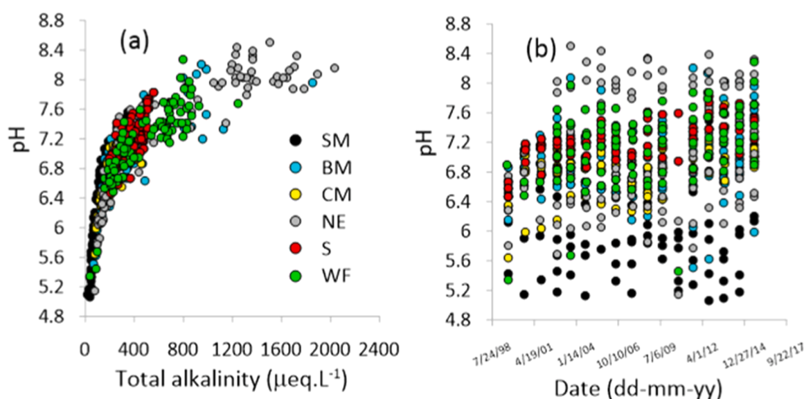
Fig. 2. (a) Total Alkalinity (left) and time (right), (b) as a function of pH for the RAMP Lakes.
