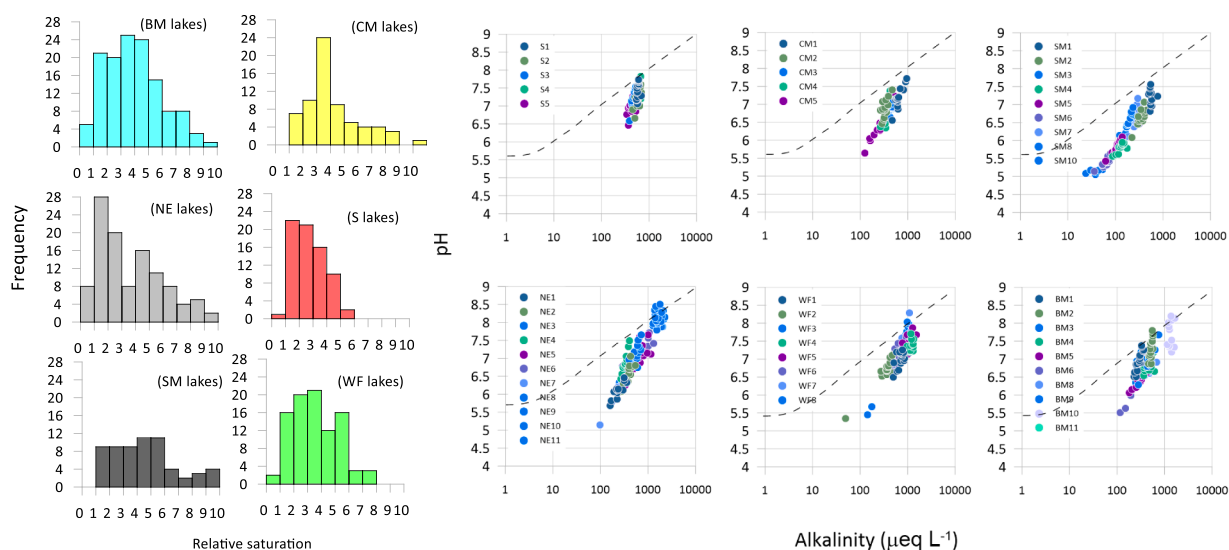
Fig. 6. \text{CO}_2 relative saturation of lakes with respect to atmospheric concentration (left) and pH alkalinity and apparent dissolved \text{CO}_2 in RAMP lakes (right). The dashed line represents the theoretical equilibrium with the atmosphere at 20^\circ\text{C} (after Cole and Prairie, 2009). Most lakes are super-saturated (below the line however all lakes subregions seem to be trending towards atmospheric equilibrium suggesting that the atmospheric and dissolved \text{CO}_2 are buffered by the acid neutralization capacity of the alkalinity). To note several lakes in the NE, WF and BM subregions fall above the theoretical equilibrium line whereas lakes from the CM subregion fall clearly below the line.
