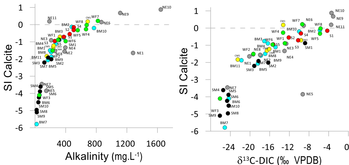
Fig. 8. Calcite saturation in relation to alkalinity or TCA (left) and in relation to \delta^{13}C_{DIC} under lakes summer conditions (June to October 2013).
