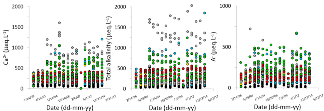
Fig. 3. Calcium, total alkalinity and A - (µeq. L -1 ) as a function of time for the RAMP Lakes.
