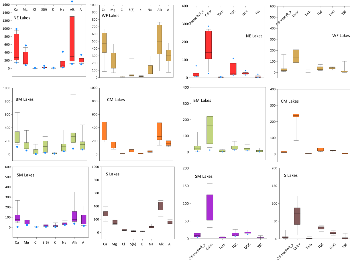
Fig. 4. RAMP Lakes Major ion concentrations (µeq.L -1 ) and physico-chemical characteristics (mg.L -1 ). Note: Chlorophyll_a in µg/L and turbidity in NTU. Lakes groups are SM -Stony Mountains, WF-West Fort McMurray, NE-Northeast Fort McMurray, BM-Birch Mountains, CM-Caribou Mountains, S – Shield. Number of sites per group of lakes is as follows: SM (n = 10), WF (n = 8), NE (n = 8), BM (n = 10), CM (n = 5), S (n = 5). The lower box boundary is 25th percentile, the line in the box is the median and the top box line is the 75th percentile. The error bars below and above represent the 10th and 90th percentile with outliers in blue circles; S(6) = SO 4 2- .
