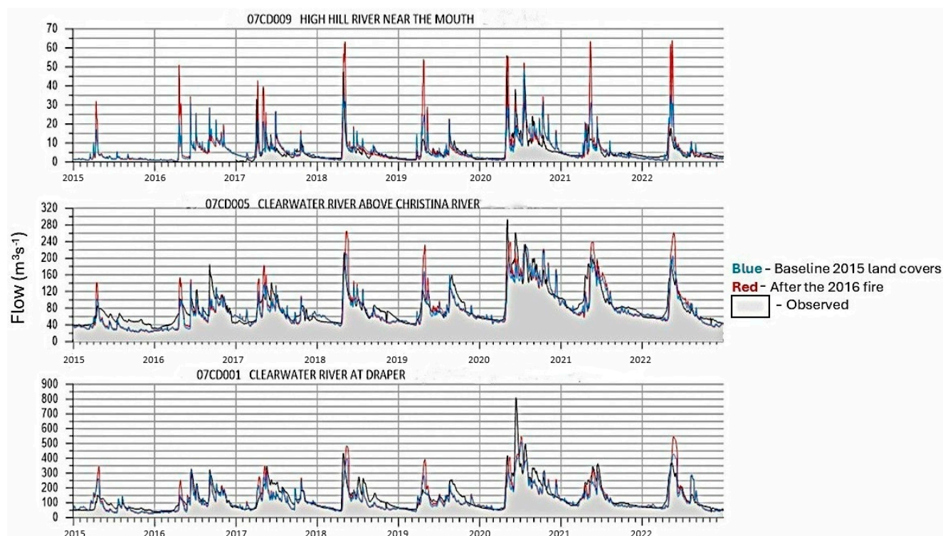
Figure 15. Hydrographs comparing baseline and post-fire response during representative events.
