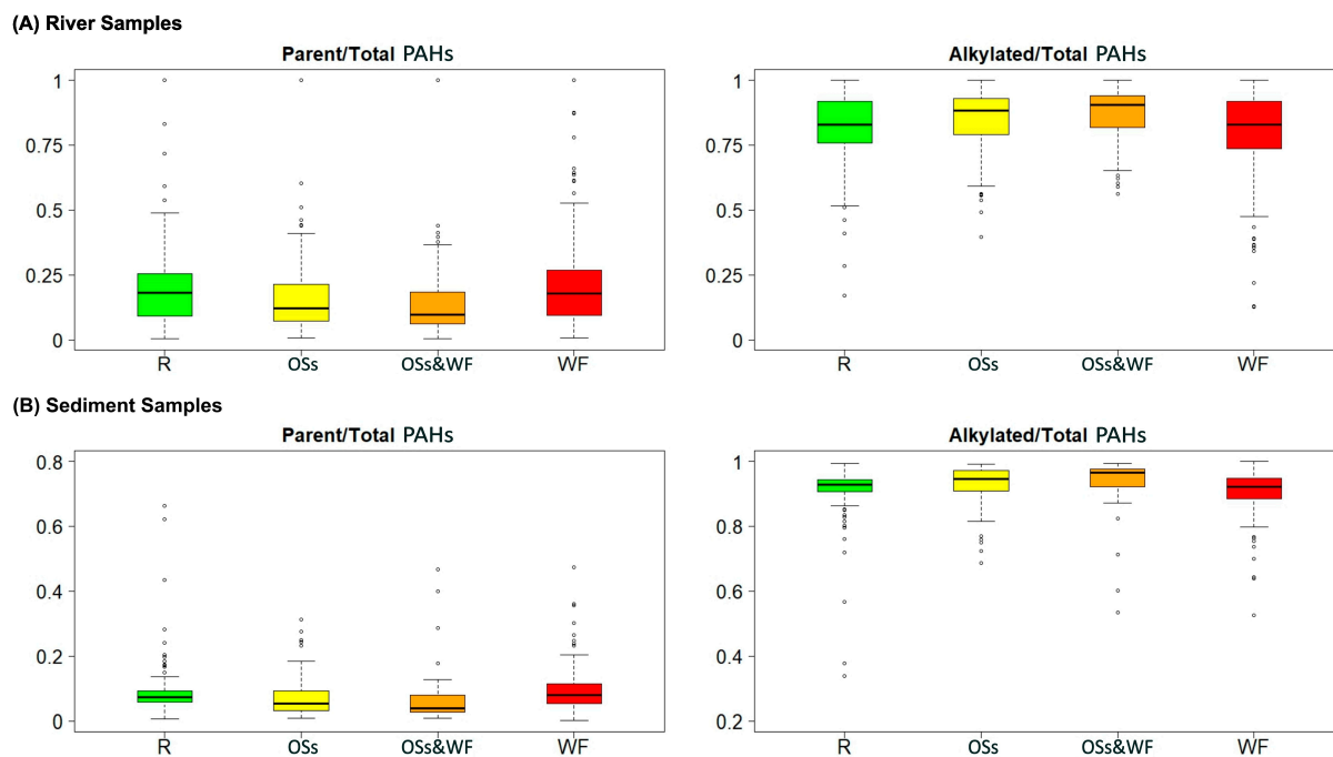
Figure 7. Box plots showing the distribution of the ratio of parent/total PAHs and alkylated/total PAHs for (A) river and (B) sediment samples, categorized by site classification (R = reference, OSs = oil sands, OSs&WF = oil sands and wildfire, and WF = wildfire). The central line indicates the median, the box represents the interquartile range, and the whiskers extend to values within 1.5 times the interquartile range. Outliers are shown as data points outside this range.
