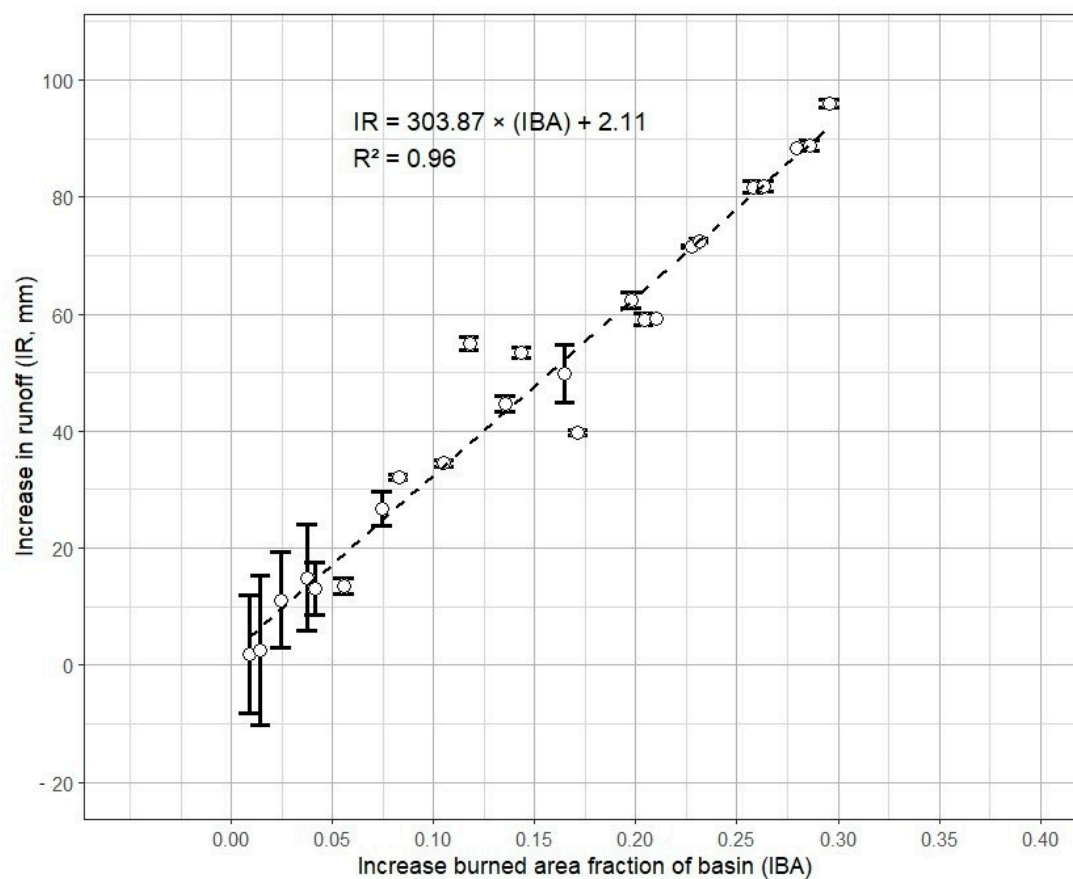
Figure 14. Relationship between burned area fraction and runoff increase (mean \pm 1 SD).
