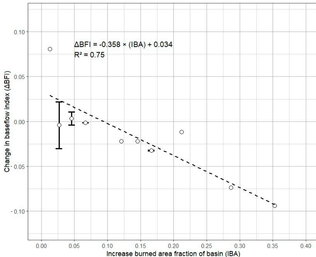
Figure 17. Change in baseflow index (BFI) as a function of burned area fraction (mean \pm 1 SD).
