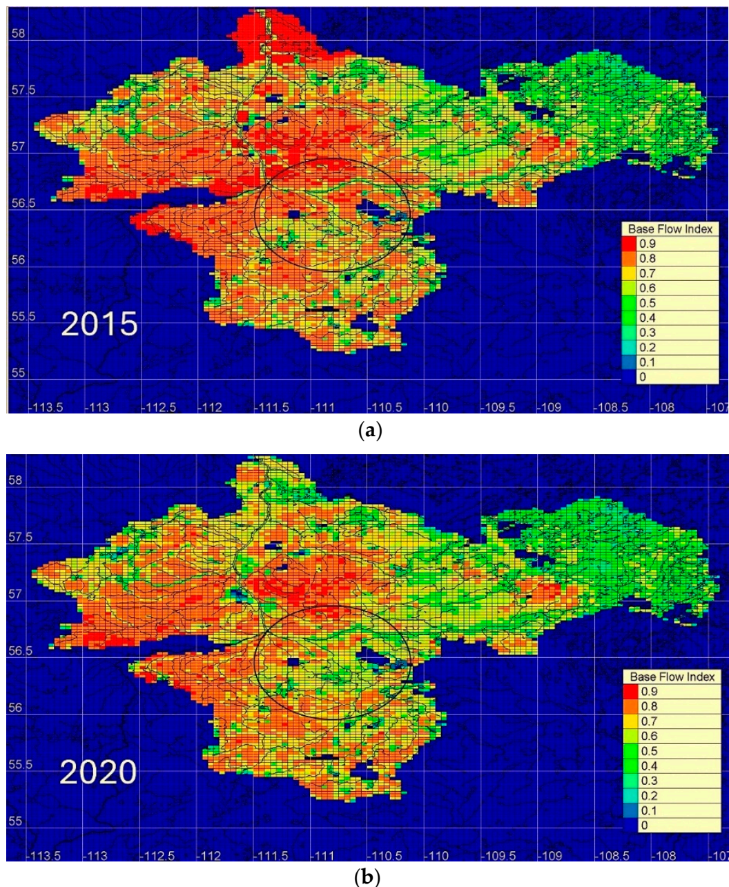
Figure 16. Spatial distribution of the BFI before (a) and after (b) wildfire, with the circled region indicating the approximate area affected by the 2016 Horse River (“The Beast”) Fire.
