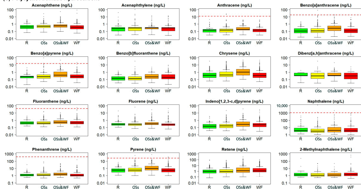
Figure 2. Box plots showing the distribution of physical–chemical parameters, metals, and PAHs for water samples, categorized by site classification (R = reference, OSs = oil sands, OSs&WF = oil sands and wildfire, and WF = wildfire). The central line indicates the median, the box represents the interquartile range, and the whiskers extend to values within 1.5 times the interquartile range. Outliers are shown as data points outside this range. The y -axis is on a logarithmic scale, and the PAH guideline values are indicated by the red dashed line (when available).
