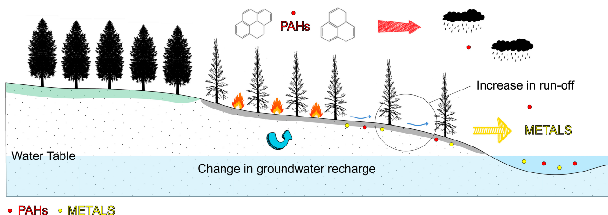
Figure 6. A conceptual model synthesizing observed patterns and inferred pathways for the transport and fate of polycyclic aromatic hydrocarbons (PAHs) and metals in water and sediment following a wildfire. Blue arrows represent run-off and groundwater recharge, red arrows represent transport of PAHs, and yellow arrows represent mobilization of metals.
