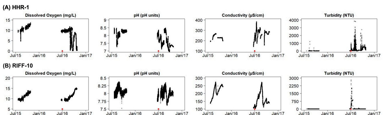
Figure 18. Time series of dissolved oxygen, pH, conductivity, and turbidity for two monitoring locations (HHR-1 and RIFF-10), with the red line indicating the date of the wildfire in the region.
