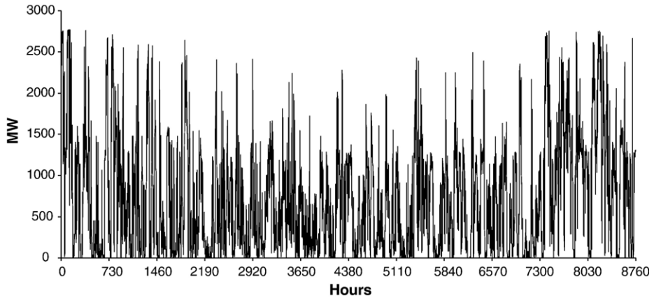
Fig. 1. Estimated power generation from two wind farms with combined capacity of 2800 MW.
