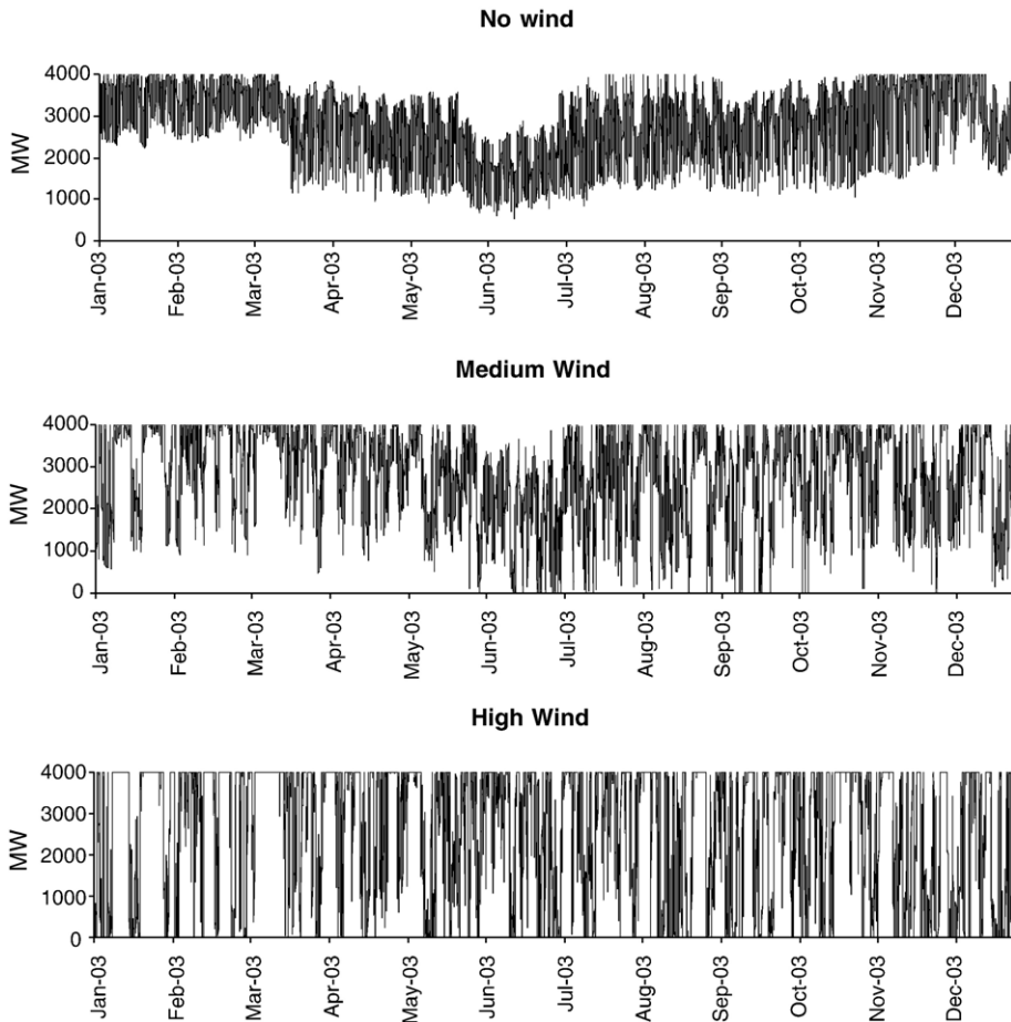
Fig. 4. Electricity dispatched by the (combined cycle) gas fired power plant, single wind farm model.
