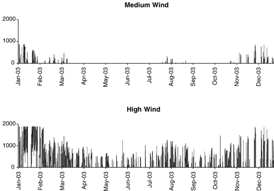
Fig. 5. Electricity dispatched by the new peak power generator, single wind farm model.
