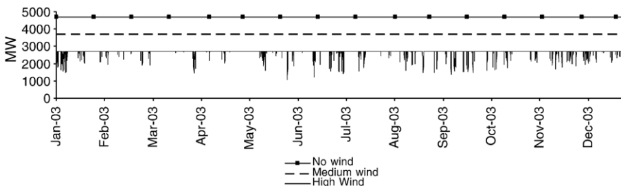
Fig. 3. Electricity dispatched by the coal power plant in the single wind farm model.
