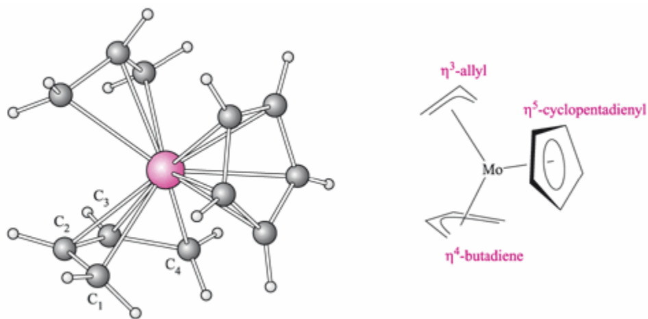
Structure of \text{Mo}(\eta^3\text{-C}_3\text{H}_5)(\eta^4\text{-CH}_2\text{CHCHCH}_2)(\eta^5\text{-C}_5\text{H}_5) .
