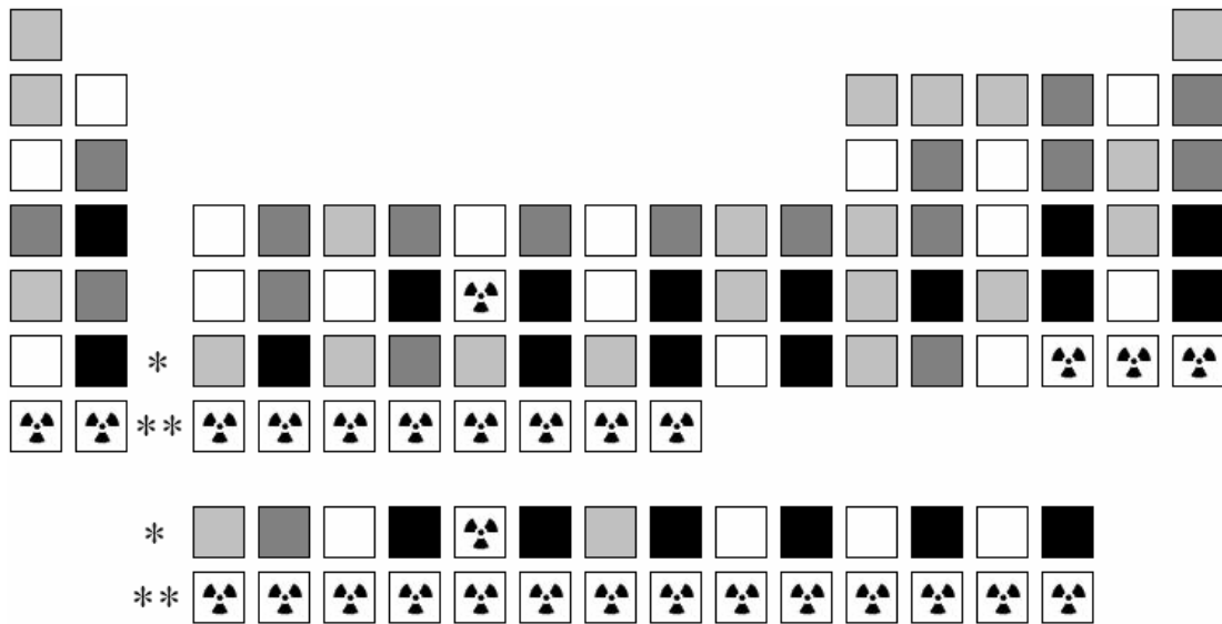
Figure 7.1 The periodic table of the elements colored by number of isotopes (white = 1 isotope, grey = 2, dark grey = 3-5, black = 6+; symbol = all isotopes are radioactive)
