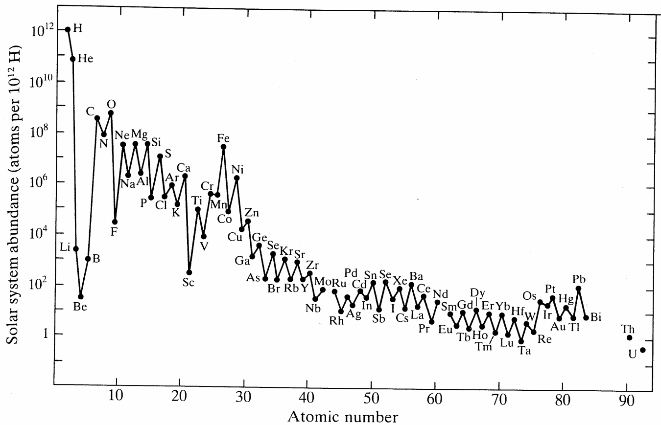
Figure 7.3 Solar system abundances of the elements, showing the relative number of atoms based on a logarithmic scale, normalized to the value 10^{12} for H.
