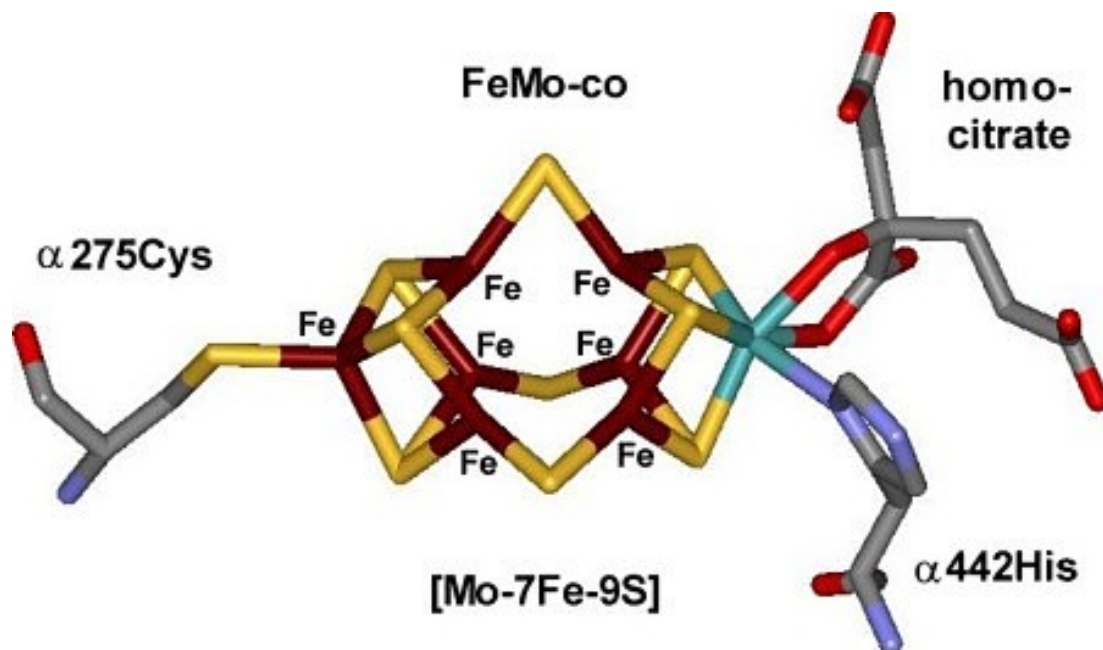
Figure D.2 Protein bound iron-molybdenum-cofactor.
