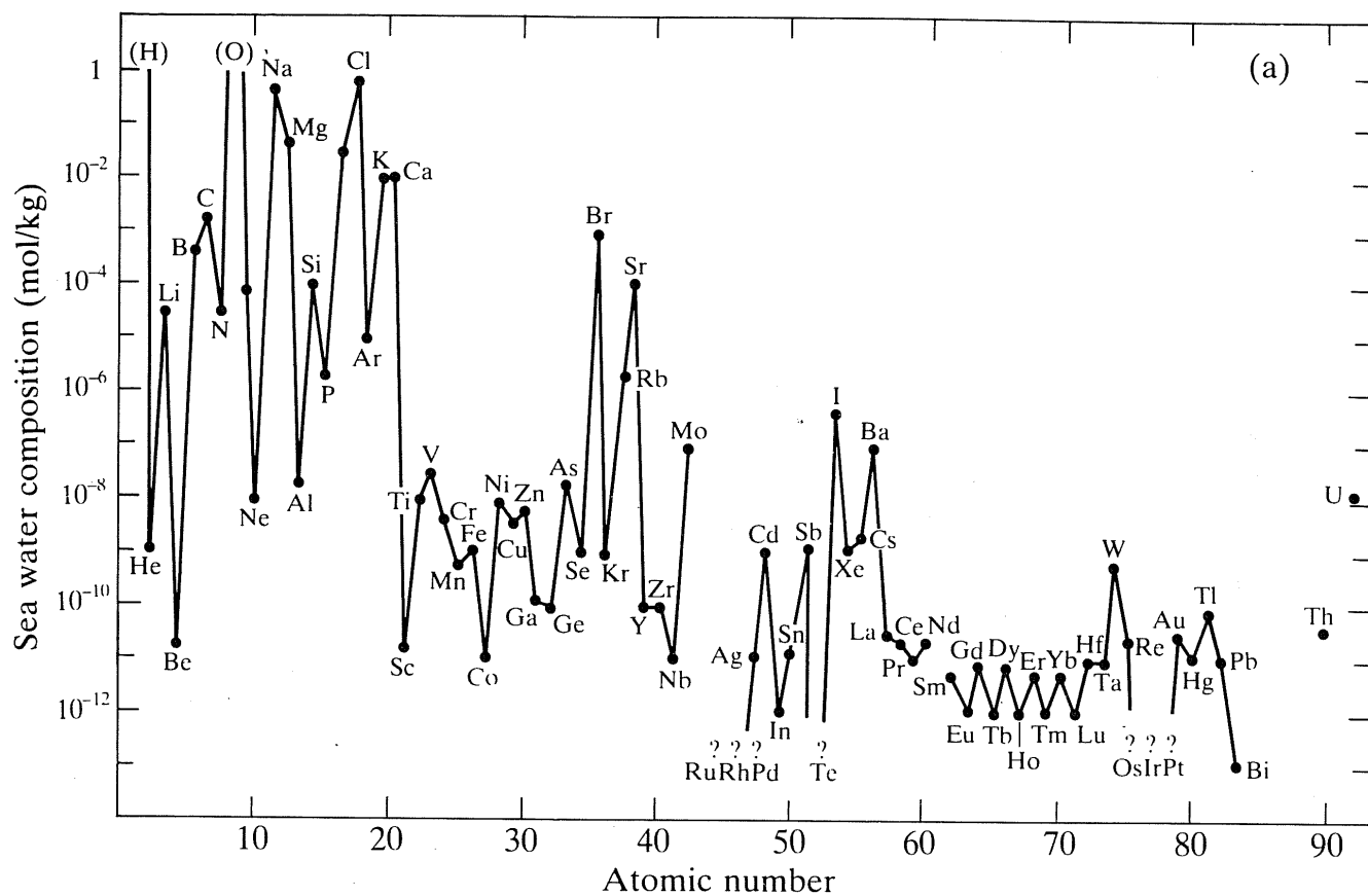
Figure D.3 Elemental abundances in the oceans; conc. of dissolved species in seawater.
