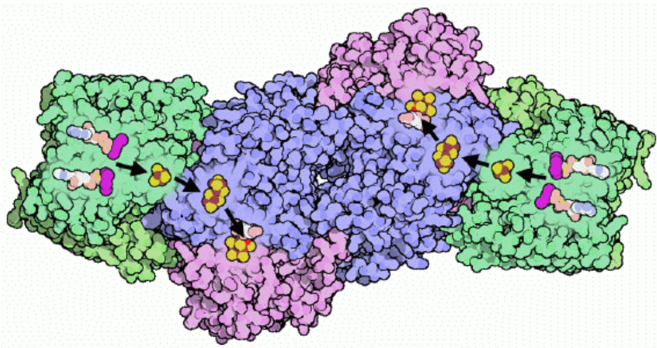
Figure D.1 The structure of nitrogenase isolated from Azotobacter vinelandii .
