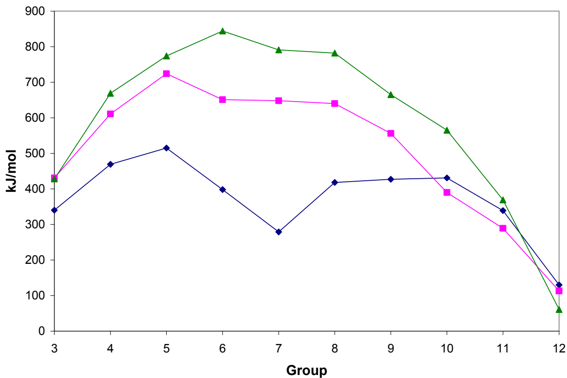
Figure 4.1 Atomization enthalpies of the d-block metals
