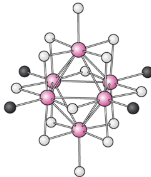
Figure 4.3 The structure of [Zr_6Cl_{14}(PPR_3)_4]
