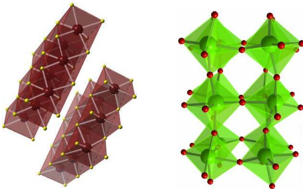
Figure 6.2 Crystal structures of MoS 2 (left) and WO 3 (right).
