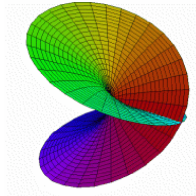
Manifold data
