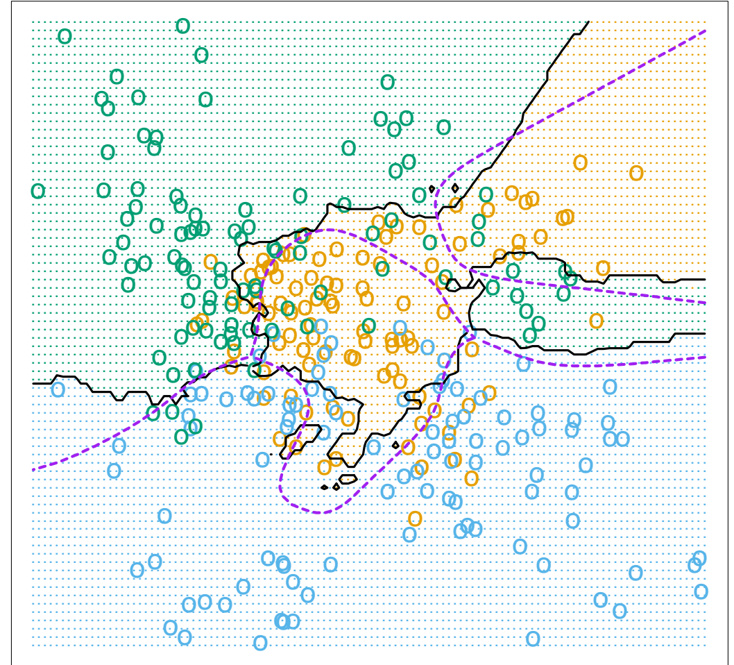
15-Nearest Neighbors
