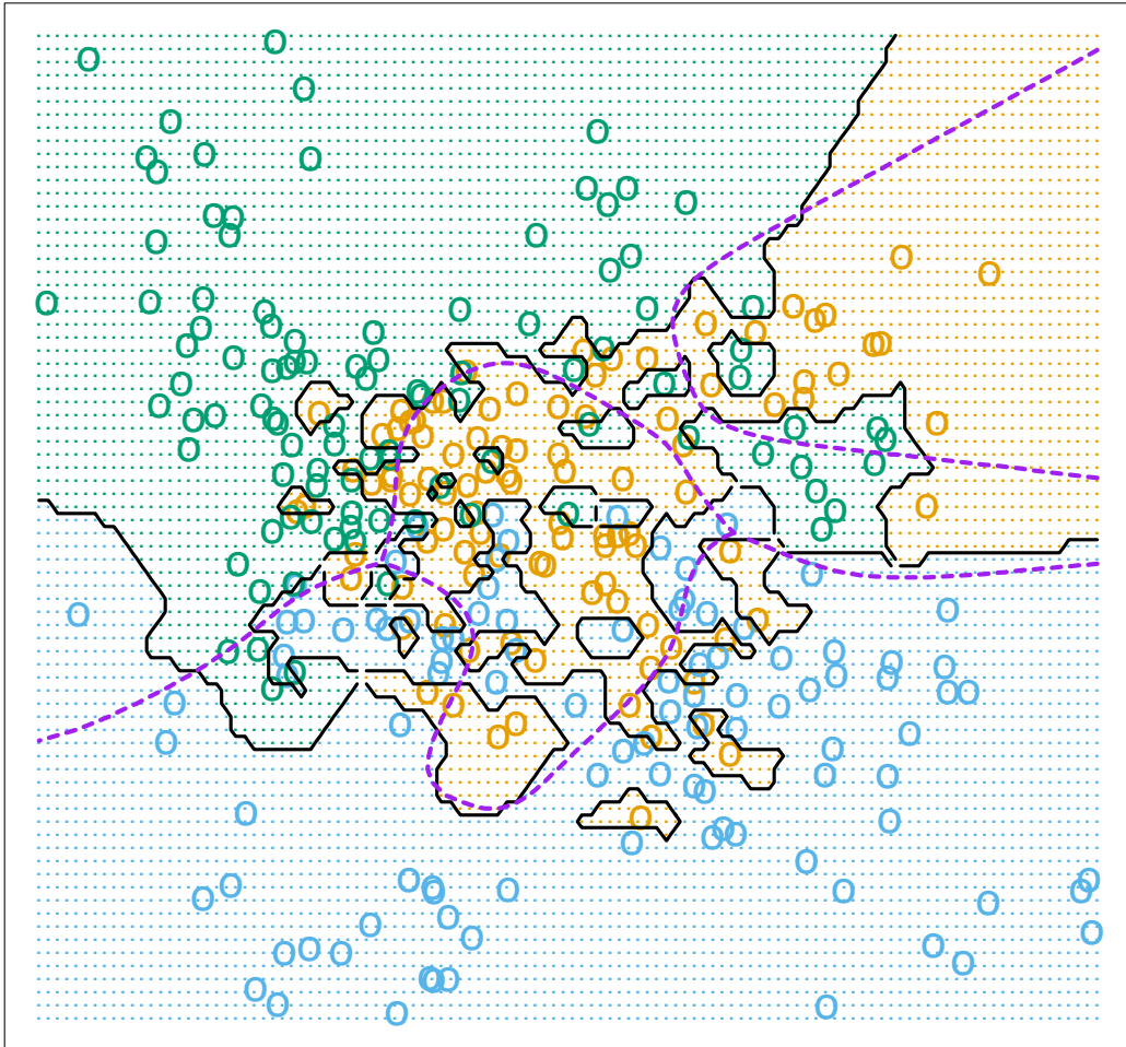
1-Nearest Neighbor
