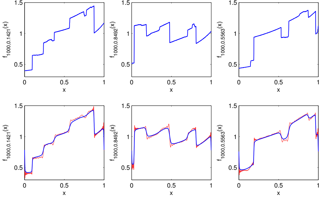
FIGURE 2. Estimates f_{k,\sigma^j\omega} , \omega = 0 , j = 20, 21, 22 using Ulam's method (upper row) and Fejér kernels (lower row, thick [blue, online]). The pure Galerkin estimates using the Galerkin Fourier matrices [\mathcal{L}'_{k,\omega}] are shown as thinner [red, online] curves in the lower row.
