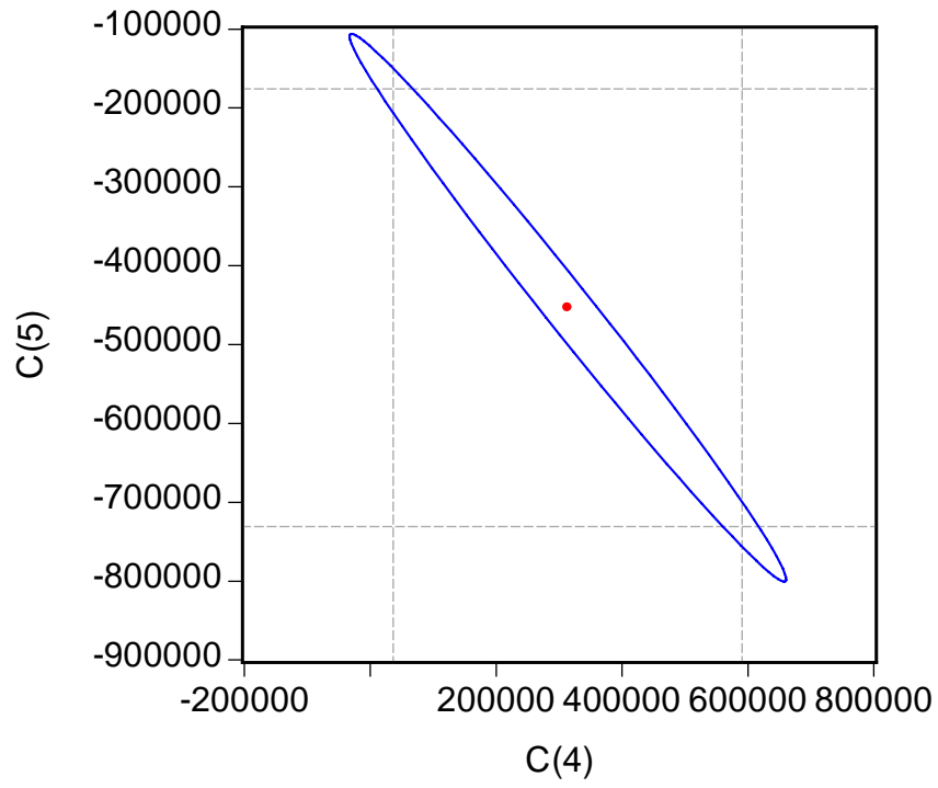
95% Confidence Ellipse
