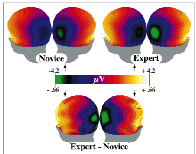
Fig. 3. Topographic distribution of the N170 expertise effect. The illustrations at the top show mean voltages from 140 to 188 ms after picture onset, separately for novice and expert domains ( 0.7 \mu\text{V} between contour lines). The illustration at the bottom shows mean voltage differences between expert and novice domains between 140 and 188 ms after picture onset ( 0.11 \mu\text{V} between contour lines).
