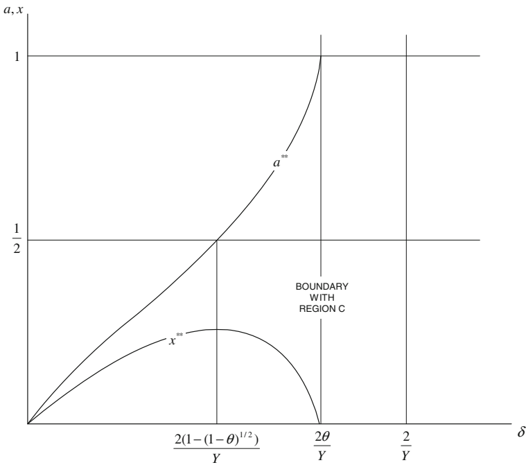
Fig. 3 The first-best solution in region A1
