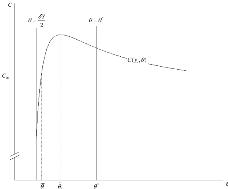
Fig. 5 The equilibrium cost function for country i
