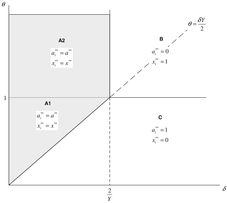
Fig. 2 The first-best solution
