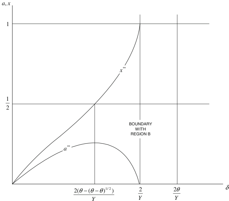
Fig. 4 The first-best solution in region A2
