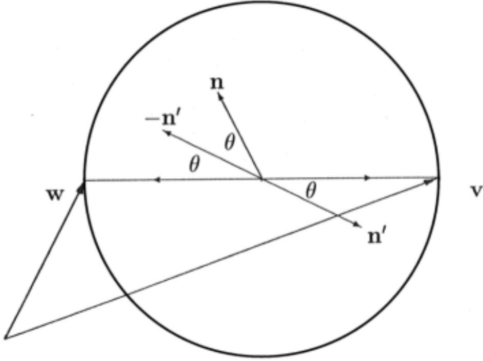
Figure 2: Geometric meanings of \mathbf{v} - \mathbf{w} , \mathbf{n} and \mathbf{n}'
