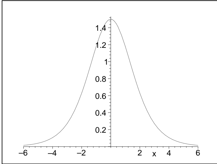
Figure 1: Equilibrium Solution for Example 2
